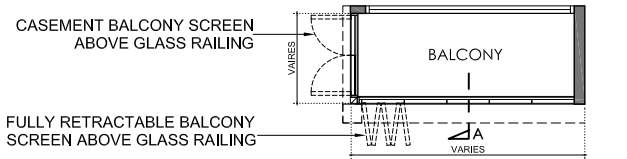
TYPICAL BALCONY PART PLAN
