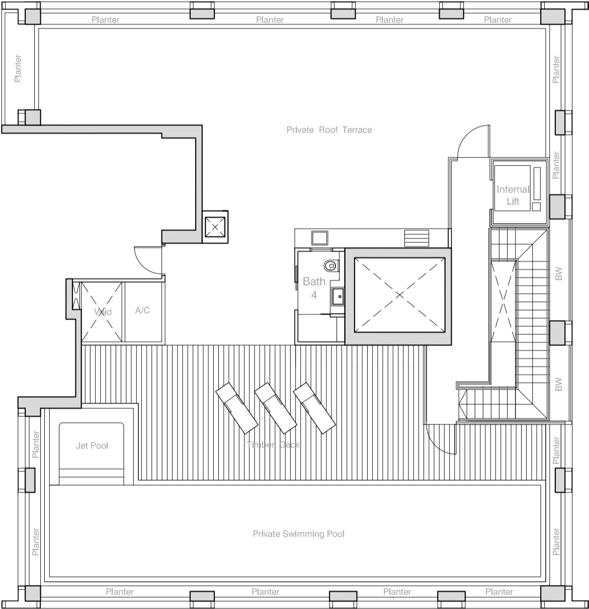
ROOF TERRACE
