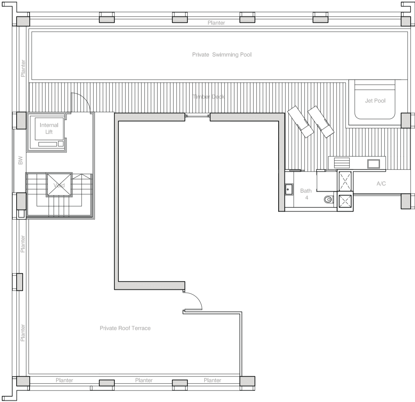
ROOF TERRACE
