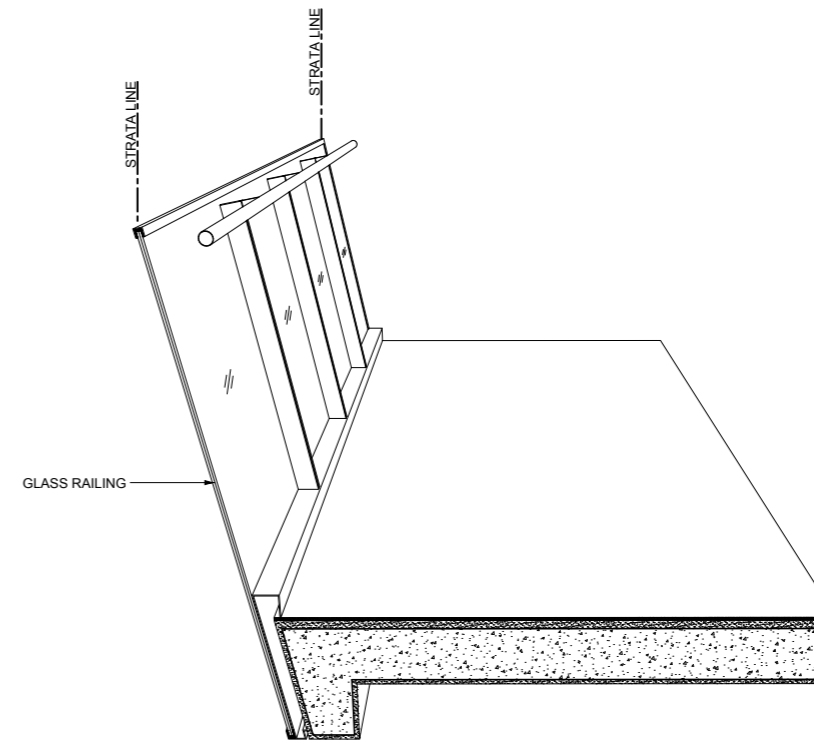
TYPICAL SECTIONAL PERSPECTIVE
