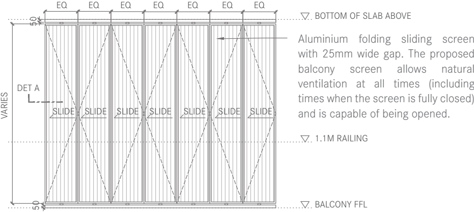
Typical Retractable Balcony Screen EI Elevation View
