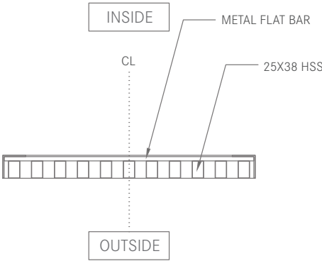
Typical Retractable Balcony Screen Detail A
