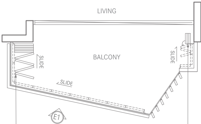
Typical Retractable Balcony Screen Plan View
